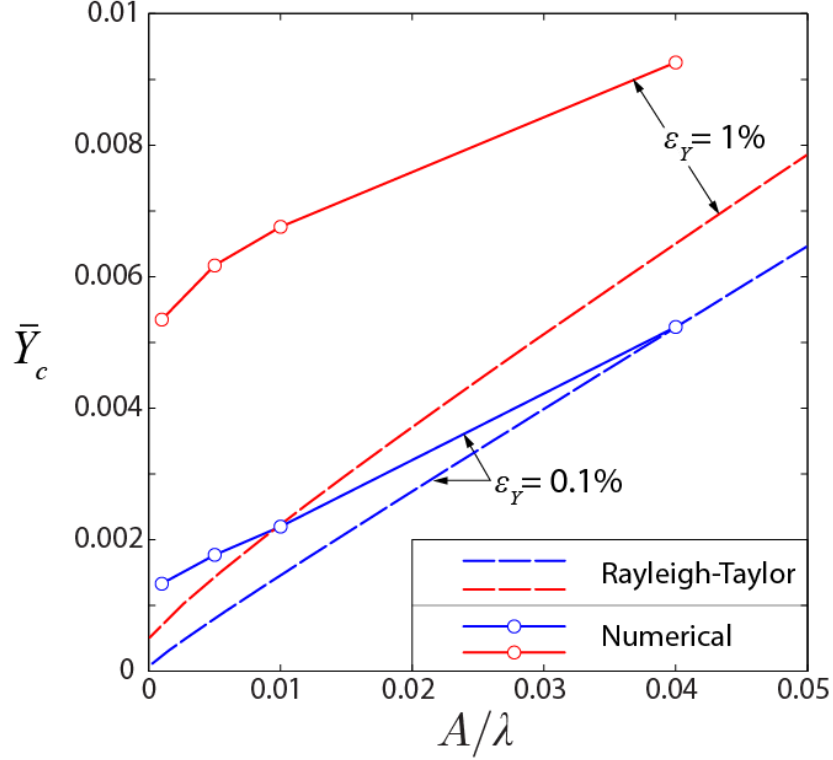
Figure 18: Comparison of direct loading and analytical Rayleigh-Taylor predictions of the variation of \bar{Y}_c with A/\lambda for frictionless slugs with \varepsilon_Y = 0.1\% and 1\% . The numerical predictions were conducted with the parameters \nu = 0.49 , D/\lambda = 3.5 , H/D = 1.4 and ramp time t_R c_L / \lambda = 50 .
