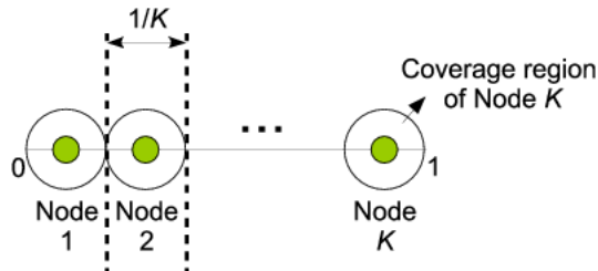
Figure 8: Schematic of backbone nodes placed along a 1-dimensional torus. The i^{\text{th}} backbone node is placed at r_i = (i - \frac{1}{2}) \frac{1}{K} from the origin, for i = 1, 2, \dots, K .
