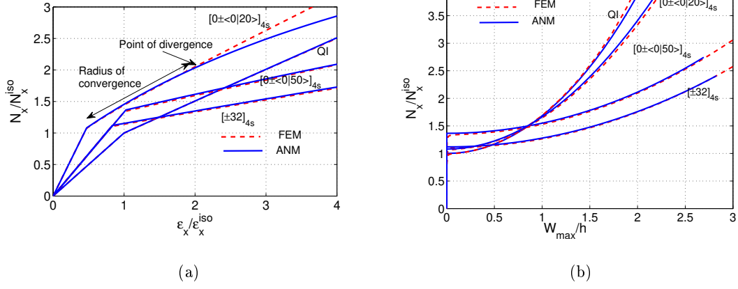
Fig. 4 ANM and FE solutions of a square simply-supported plate subjected to case B (a) Normalized axial load N_x/N_x^{iso} versus Normalized axial strain \epsilon_x/\epsilon_x^{iso} (b) Normalized axial load N_x/N_x^{iso} versus Normalized maximum transverse displacement W/h
