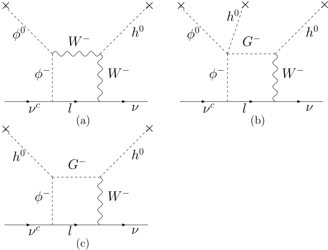
FIG. 1: Representative one-loop diagrams giving rise to neutrino masses via dimension-five operators.
