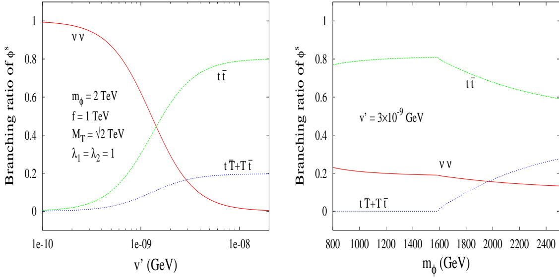
FIG. 4: Branching ratios of \phi^s (a) versus the triplet vev for Yv' = 10^{-10} GeV and m_\phi = 2 TeV, and (b) versus m_\phi for v' = 3 \times 10^{-9} GeV. The branching ratios of \phi^p are virtually identical for the parameter ranges shown.
