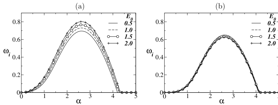
Fig. 11. Effect of the electric Weber number, E_0 on the dispersion curve ( \omega_i versus \alpha ). (a) \epsilon_r = 10, \sigma_r = 2 and (b) \epsilon_r = 2, \sigma_r = 10 . Here, m = 1 (i.e. both fluids having same viscosity) and the rest of the parameters are for Bn = 5, n = 1, h = 0.3, Re = 10 and \Gamma = 1 .
