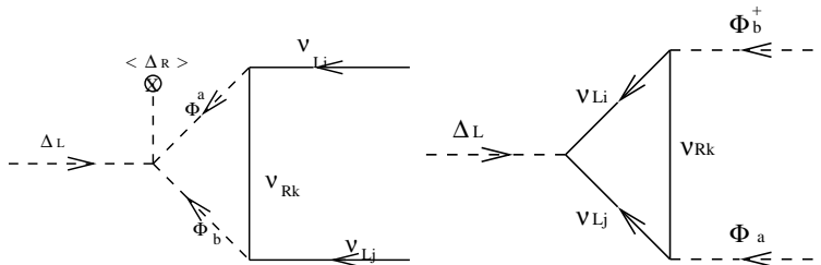
FIG. 4: The one loop radiative correction of the decay of the \Delta_L through the exchange of virtual right handed neutrinos contributing to the CP -asymmetry.
