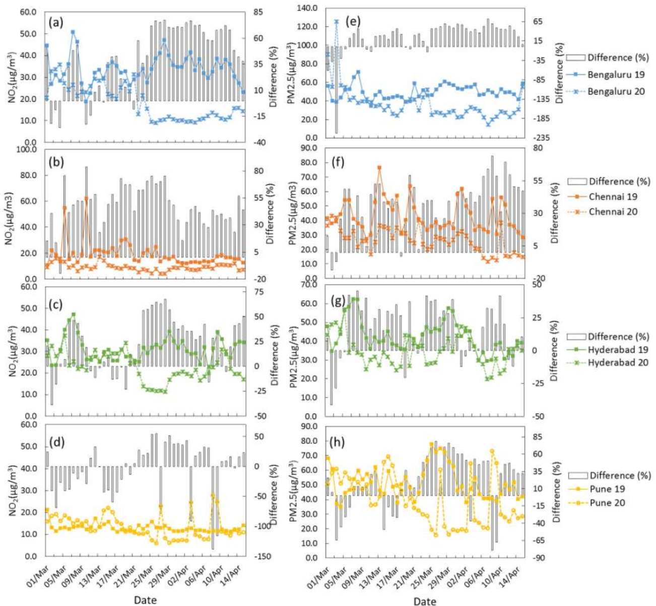
Fig. 2 \text{NO}_2 and \text{PM}_{2.5} ambient concentration in Bengaluru, Chennai, Hyderabad and Pune during the study periods of 1 st March to 15 th April for the years 2019 and 2020. Difference (%) indicates the per-
