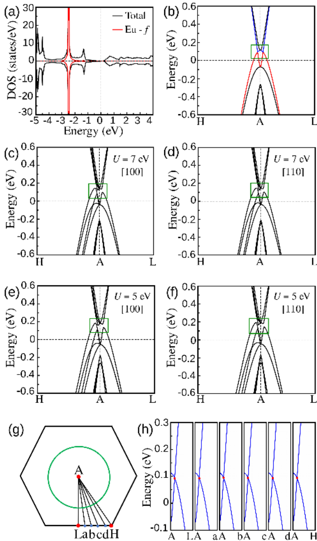
FIG. 7. (a) Total and projected density of states of EuAuAs. (b) Electronic band structure along H - A - L path without spin-orbit coupling. (c), (d) Electronic band structure along H - A - L path at U = 7 eV with SOC along [100] and [110] directions, respectively. (e), (f) Electronic band structure at U = 5 eV with SOC along [100] and [110] directions, respectively. (g) The illustration of the nodal-line, where a , b , c and d are equally spaced points between L and H . (h) Electronic band structure at different high symmetry points [as indicated in (g)] in the Brillouin zone in the k_z = 0.5 plane.
