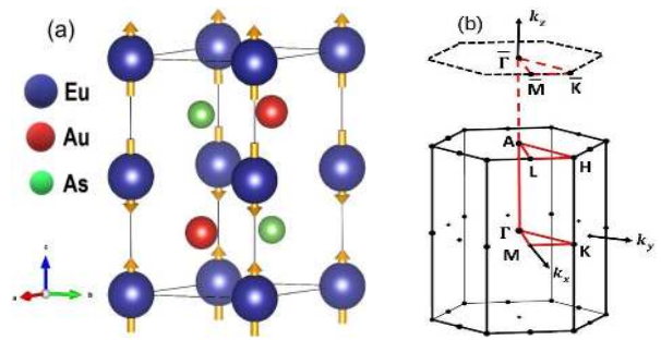
FIG. 6. (a) Crystal structure of EuAuAs and (b) the irreducible Brillouin zone of the bulk along with the (001) projected surface.
