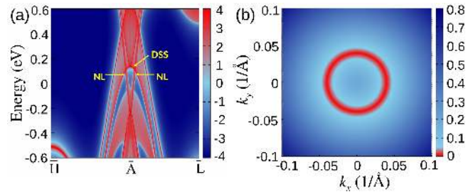
FIG. 8. (a) The surface states with Eu-termination along H - A - L path and (b) the corresponding Fermi arc in the k_z = 0.5 plane.
