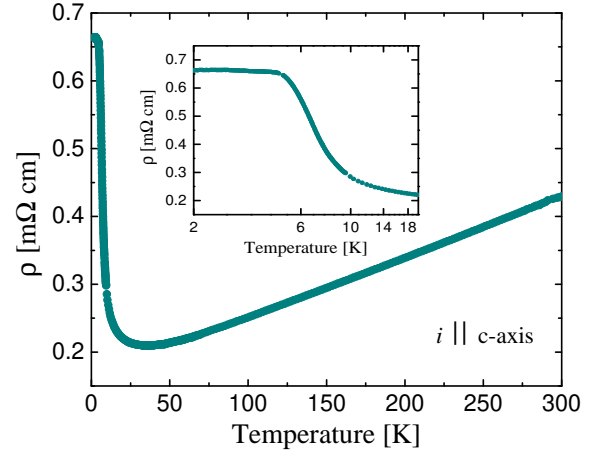
FIG. 4. Temperature dependence of the electrical resistivity of EuAuAs single crystal measured with the electric current flowing along the c axis of the hexagonal unit cell. A close view of the resistivity at low temperatures is shown in the inset (note a semilogarithmic scale).
