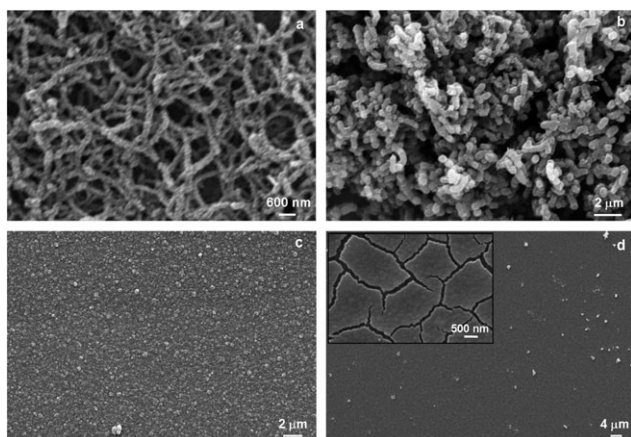
Fig. 3 SEM micrographs of the electroactive films: (a) elongated and (b) short fibers of PANI, (c) PEDOT and (d) PB used for fabricating the devices. Inset of (d) is the magnified view of PB film surface, illustrating the cracks formed on the uppermost layer of the film.
