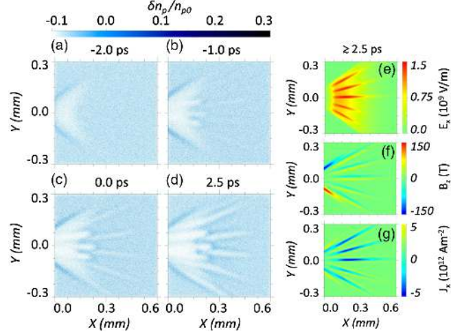
FIG. 4. (a)–(d) Synthetic proton images from qTrace simulations. Slice maps of (e) the electric E_x , (f) the magnetic field B_z and (g) the net current density J_x at saturation. In (f) red (blue) color indicates a field exiting (entering) the page and normal to it.
