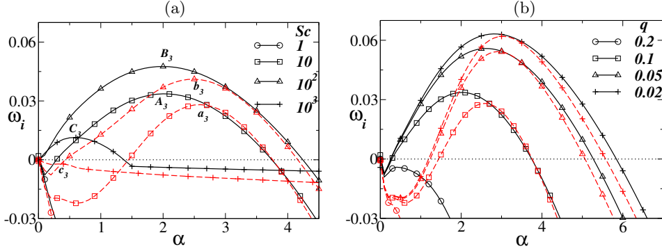
Figure 11: The effect of varying (a) Sc for q = 0.1 , and (b) q for Sc = 10 , on the dispersion curves ( \omega_i versus \alpha ). Here, solid and dashed lines represent the results for \beta = 0 and \beta = 1 , respectively. The radius of the center of the mixed region, i.e. R_1 + q/2 is fixed at 0.5. The rest of the parameter values are Re = 500 , R_s = 1 , R_f = -1.1 and \delta = 10 . The region above the dotted line ( \omega_i = 0 ) is the unstable region. The points A_3 , B_3 , C_3 and a_3 , b_3 , c_3 in panel (a) correspond to the most dangerous axisymmetric and corkscrew modes for Sc = 10 , 100 and 1000, respectively. The equivalent SC flows ( Sc_{eq} = 2Sc/(\delta + 1) , R_s = -0.1 and R_f = 0 ) are stable ( \omega_i < 0 ) for these sets of parameter values.
