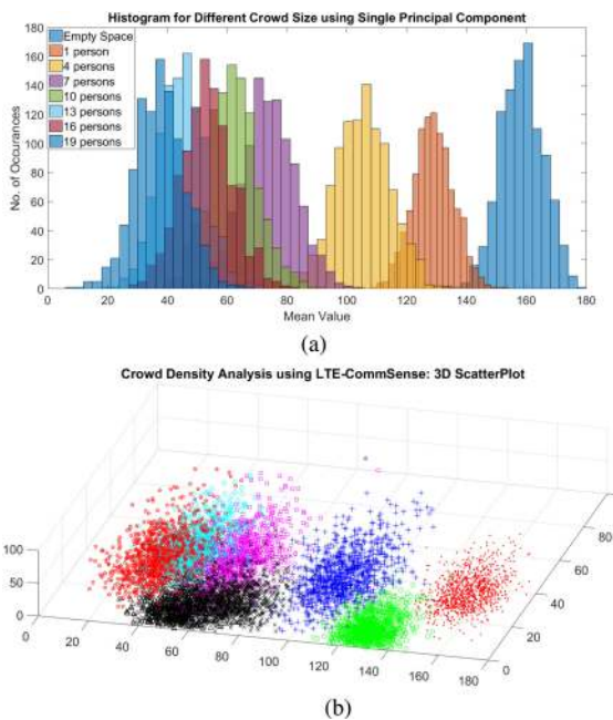
Figure 3. Dynamic crowd detection. (a) Histogram of principal component for largest eigenvalue. (b) Scatterplot corresponding to highest three eigenvalues.
