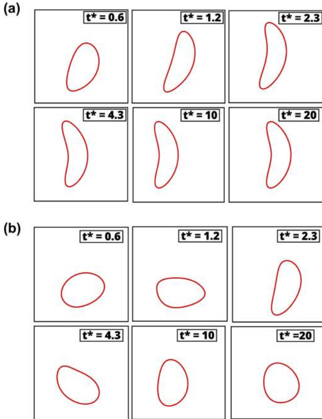
FIG. 16. The transient evolution of a drop ( a^* = 0.4 ) initially placed at y_c = -0.15 inside the channel. For system A (a) and B (b). The other parameters are Ca = 0.7 , \lambda = 1 , and E = 5 .
