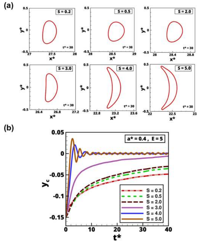
FIG. 9. Effect of varying permittivity ratio ( S = 0.2 to 5) on the deformation and migration of a drop initially placed at y_c = -0.15 . (a) The shape of a drop at t^* = 30 subjected to different permittivity ratio S . (b) The lateral position of the drop versus time. Other parameters are a^* = 0.4 , Ca = 0.7 , \lambda = 1 , and E = 5 .
