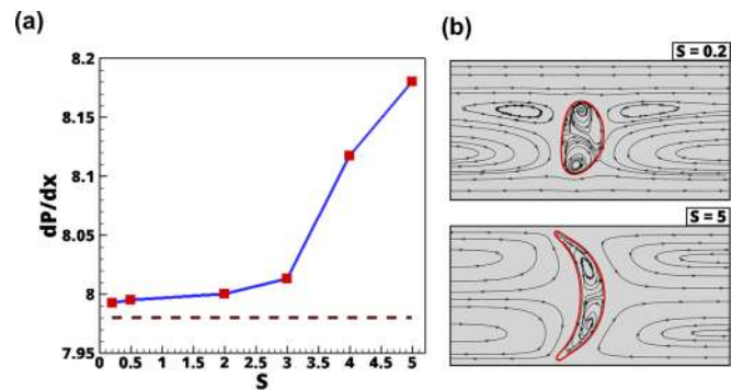
FIG. 10. Effect of elongation of the drop. (a) The normalized pressure drop in the channel for different permittivity ratio compared to the pressure drop in the channel in the absence of any drop (dashed line). (b) The streamlines around a drop subjected to varying permittivity ratio ( S = 0.2 and 5) at t^* = 30 . The flow field is presented in the frame of reference of the drop. Other parameters are a^* = 0.4 , Ca = 0.7 , \lambda = 1 , and E = 5 .
