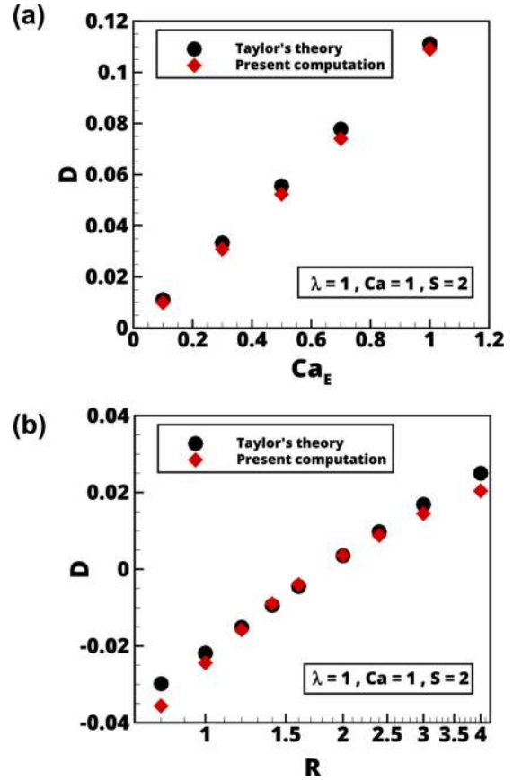
FIG. 3. Comparison of drop deformation computed from the present simulations with Taylor's theory [Eq. (16)] for varying Ca_E and R , respectively.
