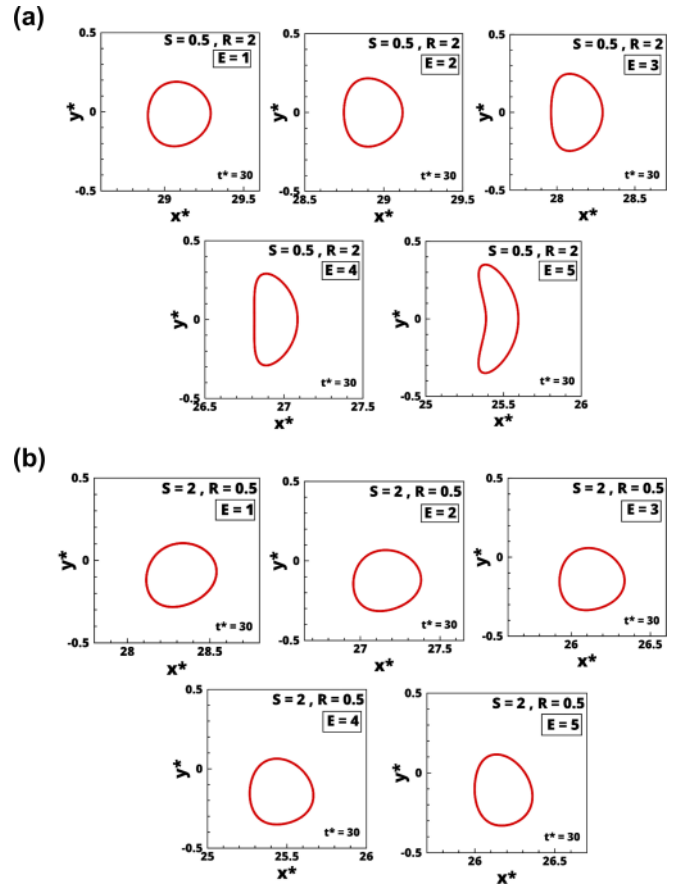
FIG. 14. Shapes of the drop at t^* = 30 while migrating from an initial off-center position of y_c = -0.15 and subjected to different permittivity ratio S , conductivity ratio R , and electric field strength E . (a) Drops suspended in a system of S = 0.5 and R = 2 and subjected to varying E . (b) Drops suspended in a system of S = 2 and R = 0.5 and subjected to varying E . E is varied in the range of 1 to 5. Other parameters are a^* = 0.4 , Ca = 0.7 , and \lambda = 1 .
