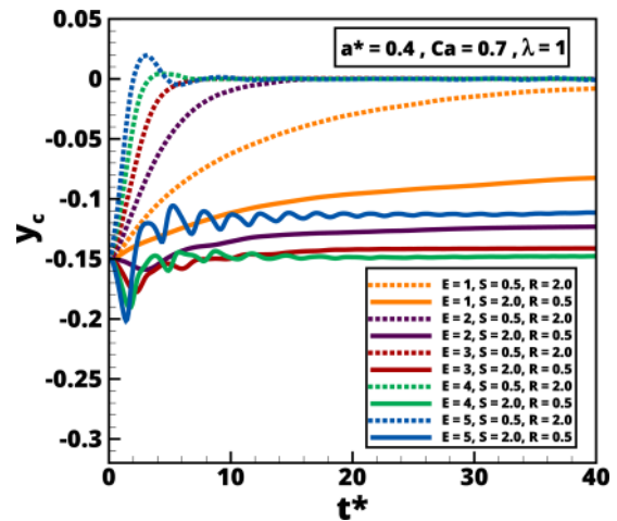
FIG. 15. The migration of a drop initially placed at y_c = -0.15 towards the center line of the channel influenced by different electric field strength E , permittivity ratio S , and conductivity ratio R . Dotted and solid lines represent the position of the drop suspended in systems A and B, respectively. Other parameters are a^* = 0.4 , Ca = 0.7 , and \lambda = 1 .
