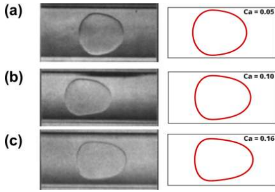
FIG. 2. Comparison of drop shape for three different Ca : 0.05, 0.10, and 0.16. The other parameters are a^* = 0.95 and \lambda = 0.99 . Left panel: Experimental results [4]; right panel: present simulations.
