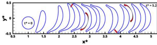
FIG. 11. Variations of shape a drop ( a^* = 0.4 ) initially placed at y_c = -0.15 inside the channel and subjected to electric field from t^* = 0 to 5.2. The other parameters are Ca = 0.7 , \lambda = 1 , E = 5 , and S = 5 .
