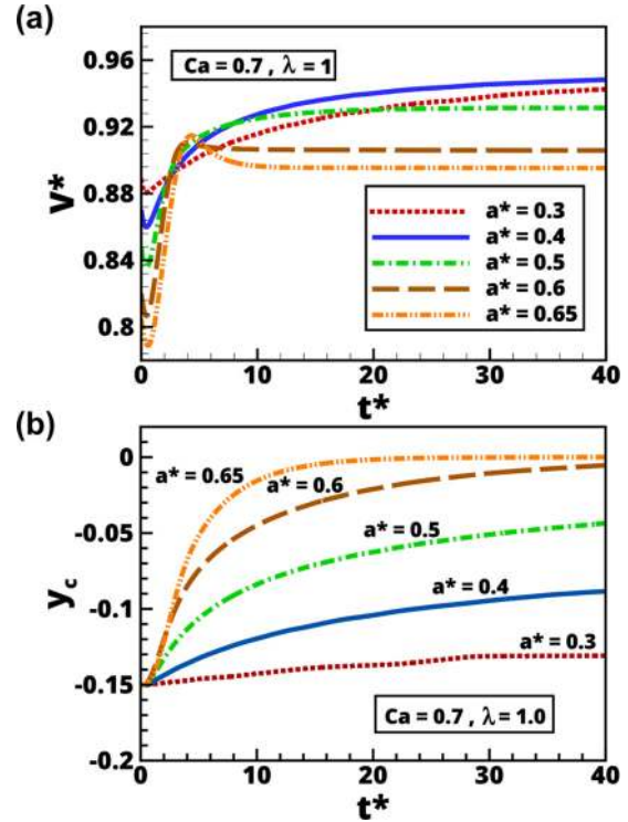
FIG. 6. Migration of different sized droplets starting from an initial off-center position ( y_c = -0.15 ) towards the channel center line. (a) Drop velocity versus time. (b) Lateral position versus time. The other parameters are Ca = 0.7 and \lambda = 1 .
