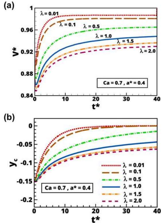
FIG. 8. The effect of varying viscosity ratio ( \lambda = 0.01 to 2.0 ) on the migration of a drop initially placed at y_c = -0.15 . (a) Drop velocity versus time. (b) Lateral position of the drop versus time. The other parameters are a^* = 0.4 and Ca = 0.7 .
