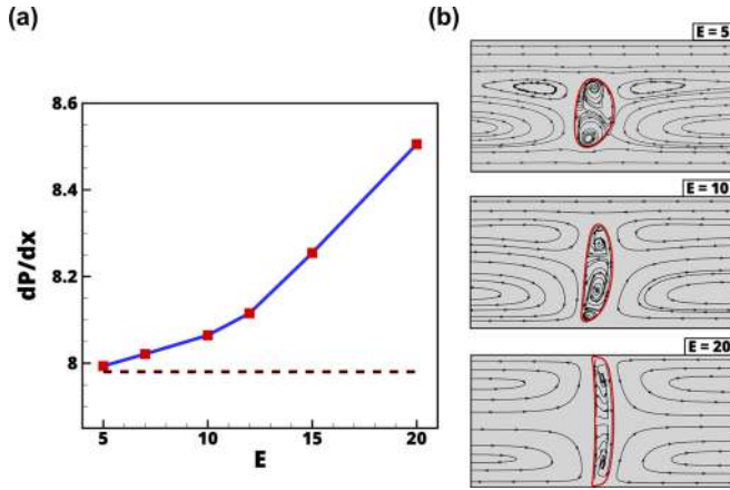
FIG. 13. Effect of elongation of the drop. (a) The normalized pressure drop in the channel for different electric field strength compared to the pressure drop in the channel in the absence of any drop (dashed line). (b) The streamlines around a drop subjected to varying electric field strength ( E = 5, 10 and 20 ) at t^* = 30 . The flow field is presented in the frame of reference of the drop. Other parameters are a^* = 0.4 , Ca = 0.7 , \lambda = 1 , and S = 0.2 .
