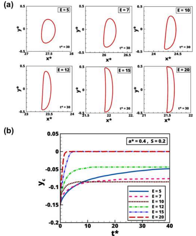
FIG. 12. Effect of varying electric field strength ( E = 5 to 20) on the deformation and migration of a drop initially placed at y_c = -0.15 . (a) The shape of a drop at t^* = 30 subjected to different E . (b) The lateral position of the drop versus time. Other parameters are a^* = 0.4 , Ca = 0.7 , \lambda = 1 , and S = 0.2 .
