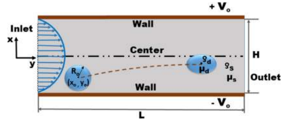
FIG. 1. The schematic representation (not to scale) of the lateral migration of a droplet inside a channel under the influence of external Poiseuille flow and uniform electric field.
