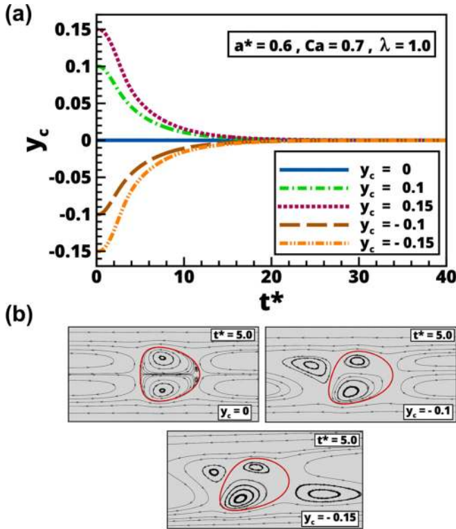
FIG. 5. A drop ( a^* = 0.6 ) initially placed at different off-center positions gradually migrates towards the center line of the channel. The other parameters are Ca = 0.7 and \lambda = 1 . (a) The lateral position of the drop versus time. (b) The streamlines around the drop placed at y_c = 0, -0.1 , and -0.15 , respectively. The flow field is presented in the frame of reference of the drop.
