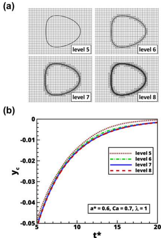
FIG. 4. Grid convergence test. (a) Snapshots of adaptive mesh generation using different levels of refinement. The refinement level of 7 is selected for the present study. (b) Comparison of y_c for different levels of grid refinement. The different parameters considered are a^* = 0.6 , Ca = 0.7 , and \lambda = 1.0 .
